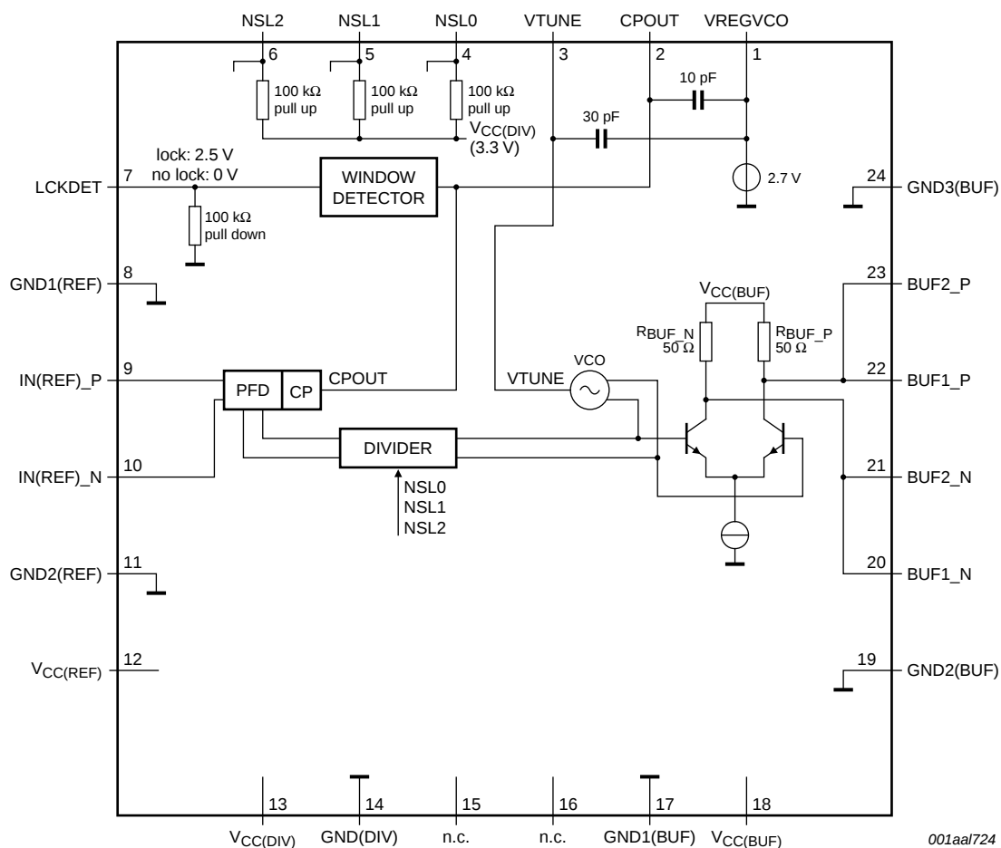
Fig 1. Block diagram
